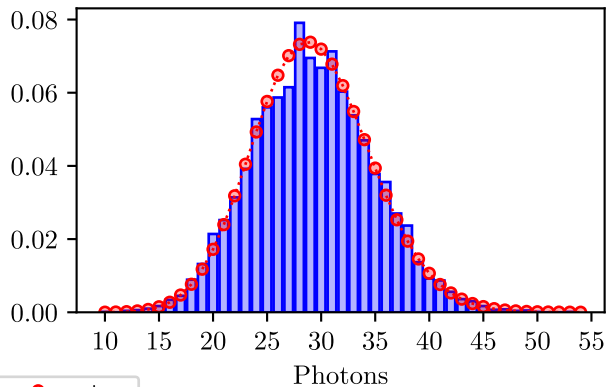
\mathcal{P}(29.2317)
