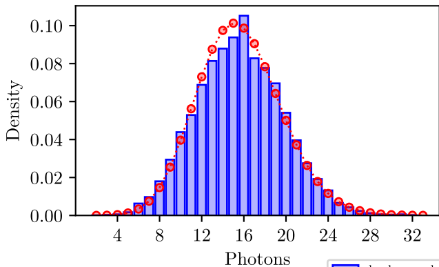
\mathcal{P}(15.5871)
